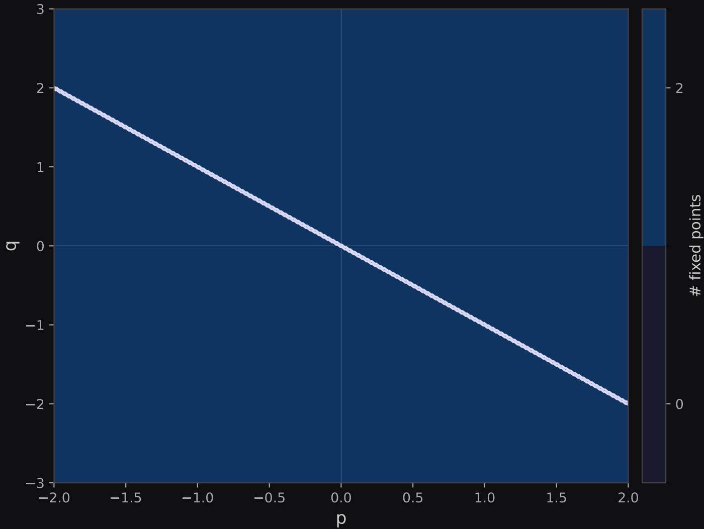
Two-parameter bifurcation diagram
